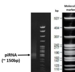
Figure 2: Representative agarose gel image of SF exosomal-TR NGS library. The 150bp bands correspond to piRNAs(30nt).
