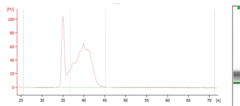
Figure 1: Representative electropherogram of SF exosomal-TR showed abundant of sncRNA.
